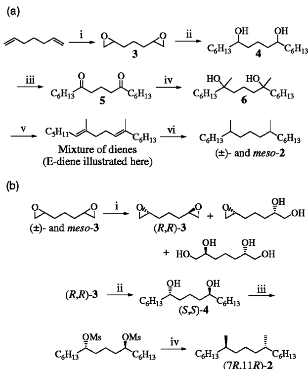
Scheme 1. (a) Synthesis of racemic 7,11-dimethylheptane, ( \pm )- and meso - 2 : (i) m -CPBA, DCM; (ii) n -pentylMgBr, CuI, diethyl ether; (iii) Jones reagent; (iv) MeMgI, diethyl ether; (v) DMSO; (vi) \text{H}_2 , Pd/C; (b) synthesis of ( R,R )- 2 : (i) [ (R,R) ]-salen \text{Co}^{\text{III}} OAc], \text{H}_2\text{O} ; (ii) n -pentylMgBr, CuI; (iii) MsCl, \text{Et}_3\text{N} ; (iv) \text{Me}_2\text{CuLi} , diethyl ether
