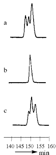
Figure 1. Enantioselective gas chromatography of 7,11-dimethylheptadecane: (a) a mixture of ( \pm ) and meso isomers; (b) ( R,R )-isomer; (c) co-injection of isomeric mixture and the ( R,R ) isomer
