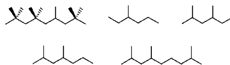
Figure 2. Examples of methylated alkanes whose enantiomers have been separated by enantioselective gas chromatography
